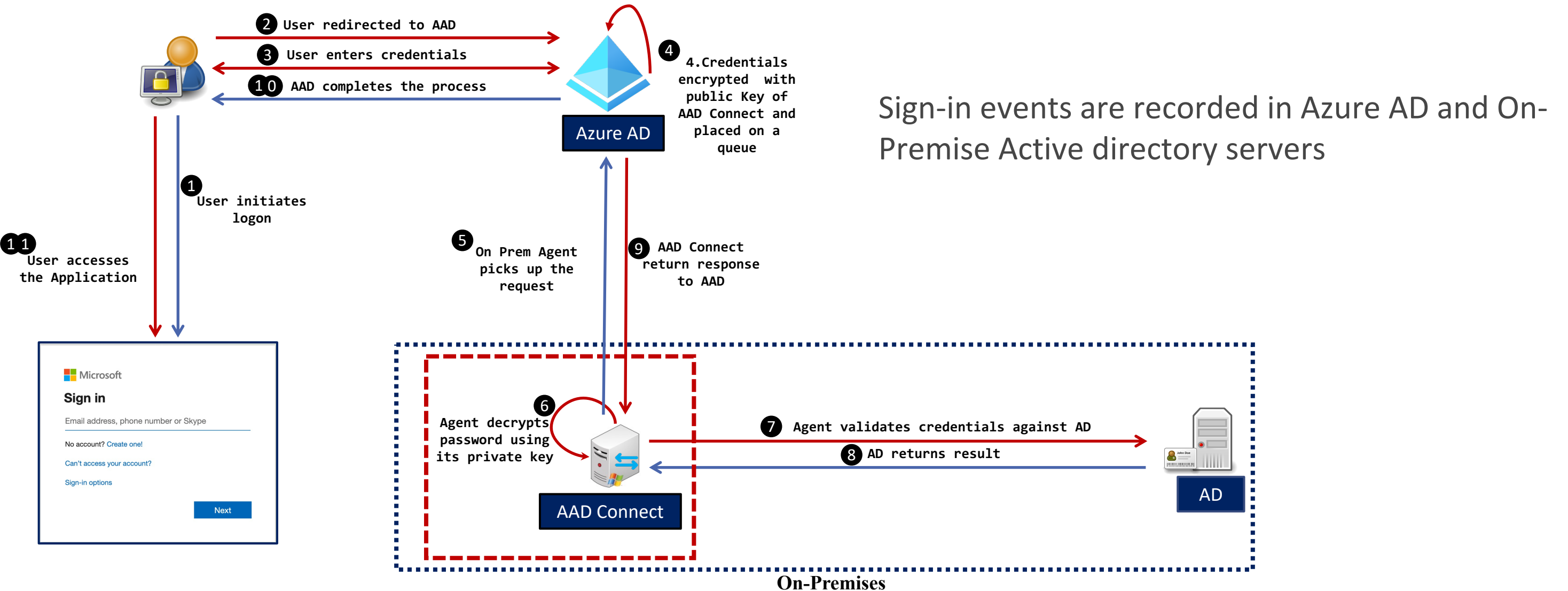
AAD Connect running Pass Through Authentication (PTA).
